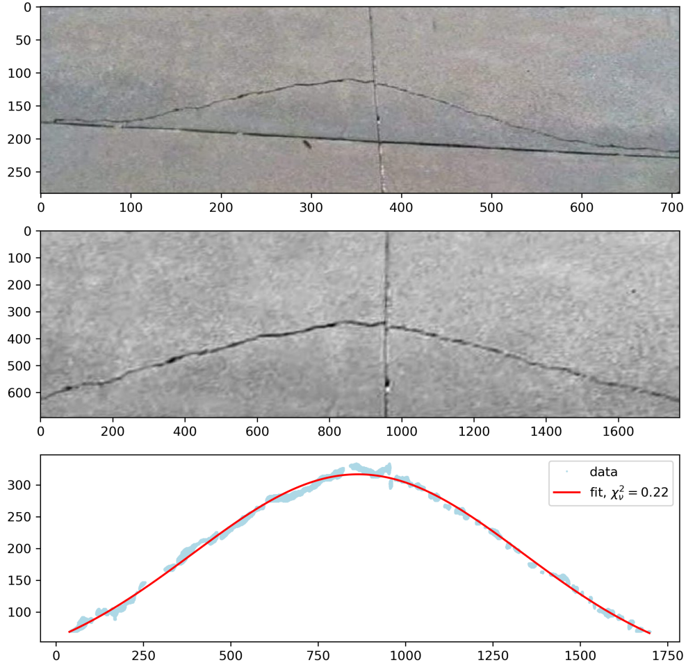
Figure 2: Top: Figure 1, Middle: Figure 1 with perspective correction and greyscale transformation, Bottom: curve fit of the sidewalk crack points
